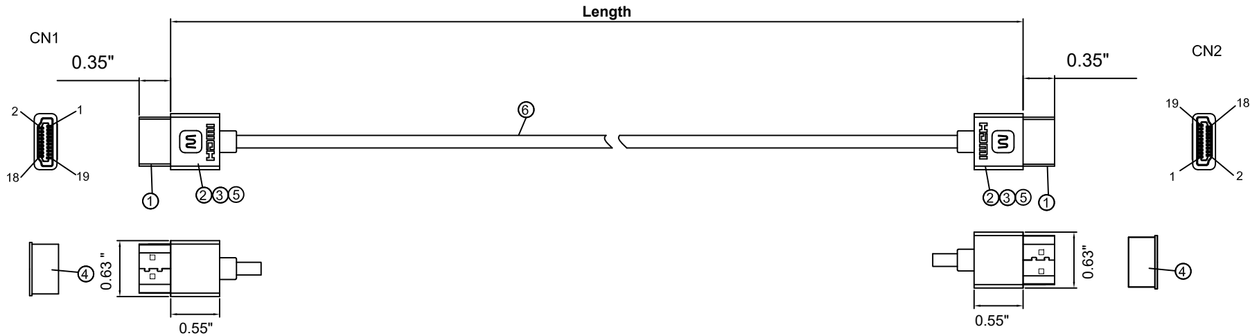
HDMI 19P/M MOLDING TYPE
